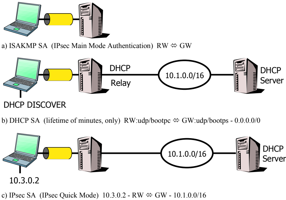
Figure 5: DHCP-over-IPsec scenario
